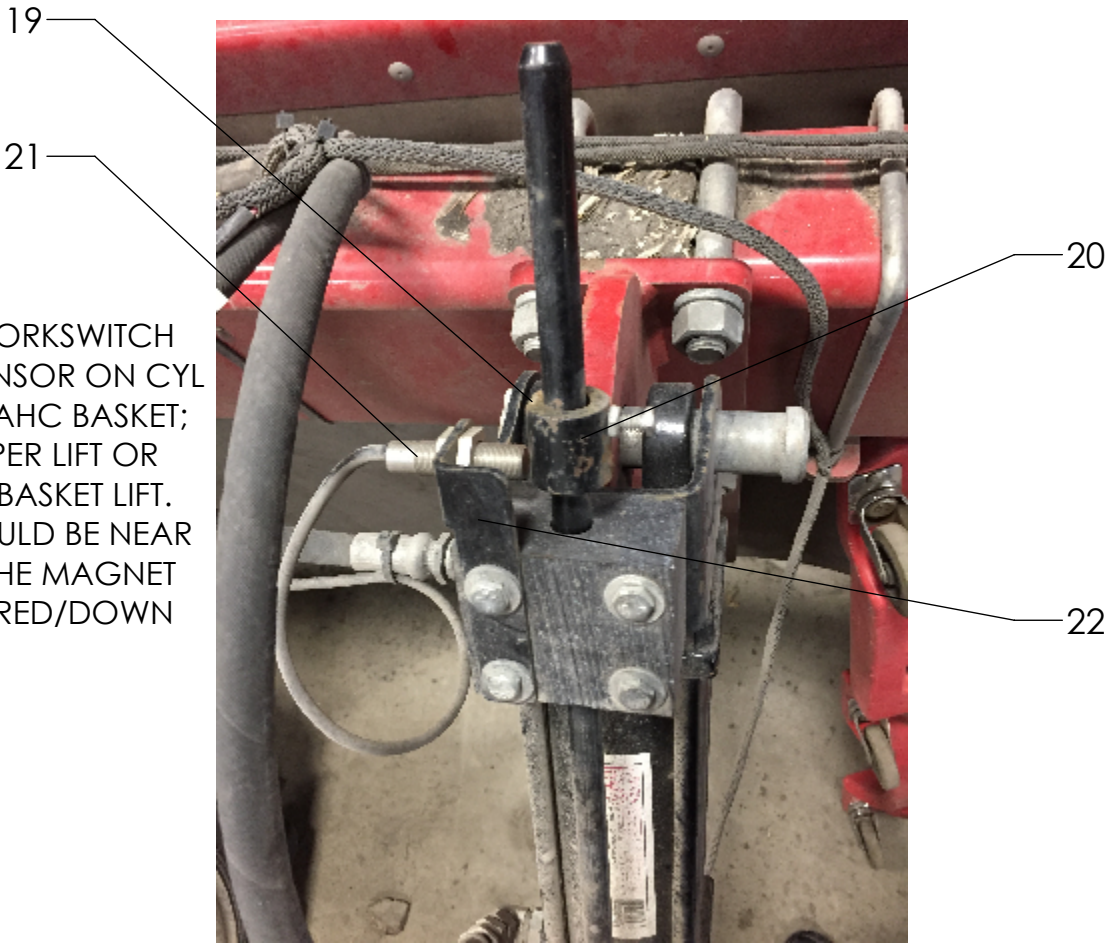
FIG. 2 - WORKSWITCH MOUNT
