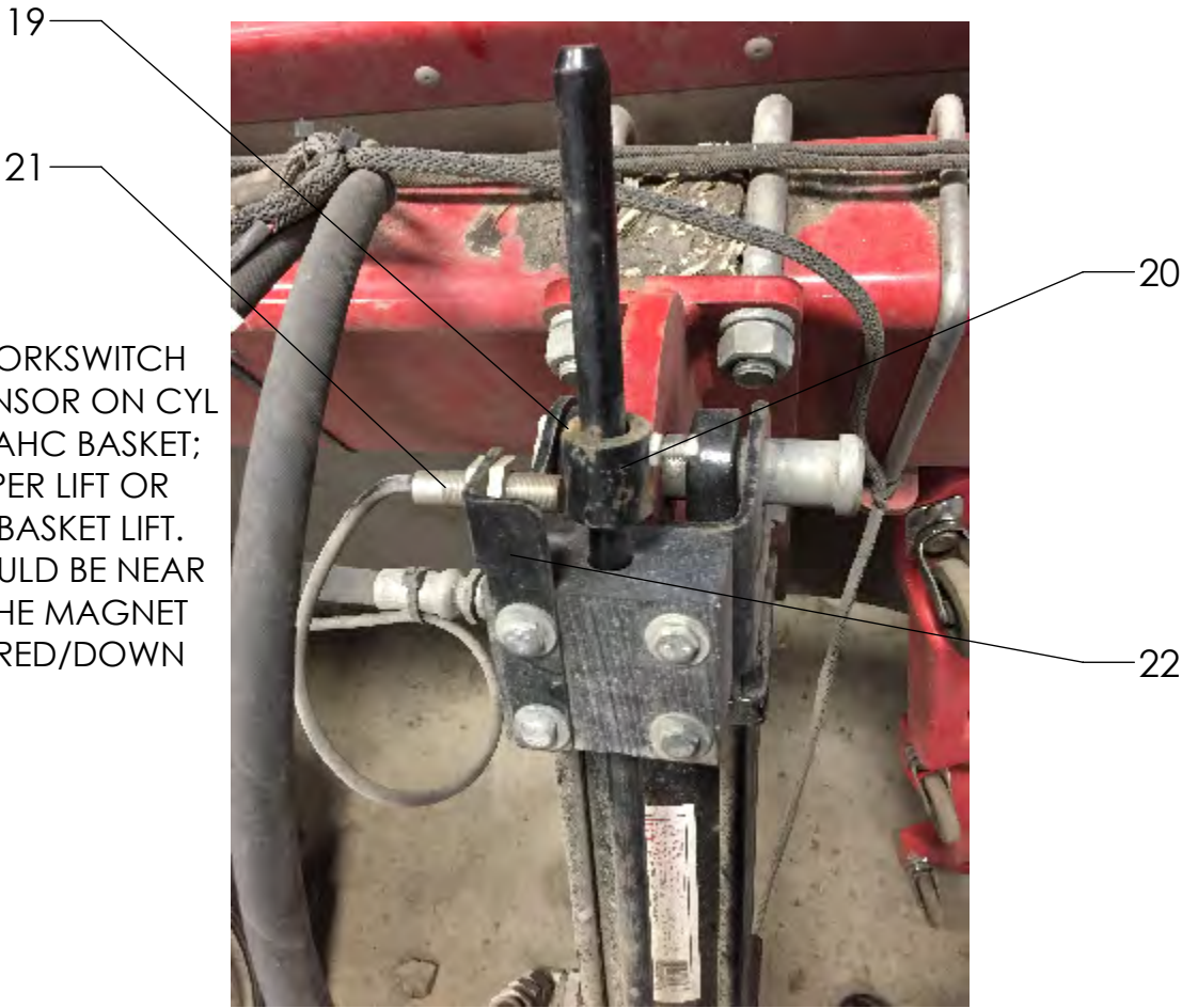
FIG. 2 - WORKSWITCH MOUNT
