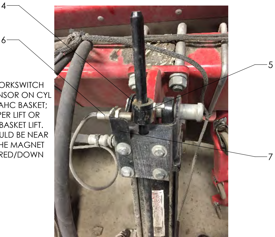
FIG. 2 - WORKSWITCH MOUNT
